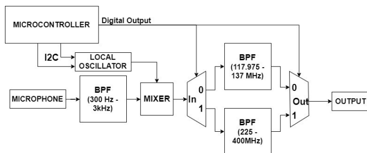
Figure 2: Transmitter Block Diagram
