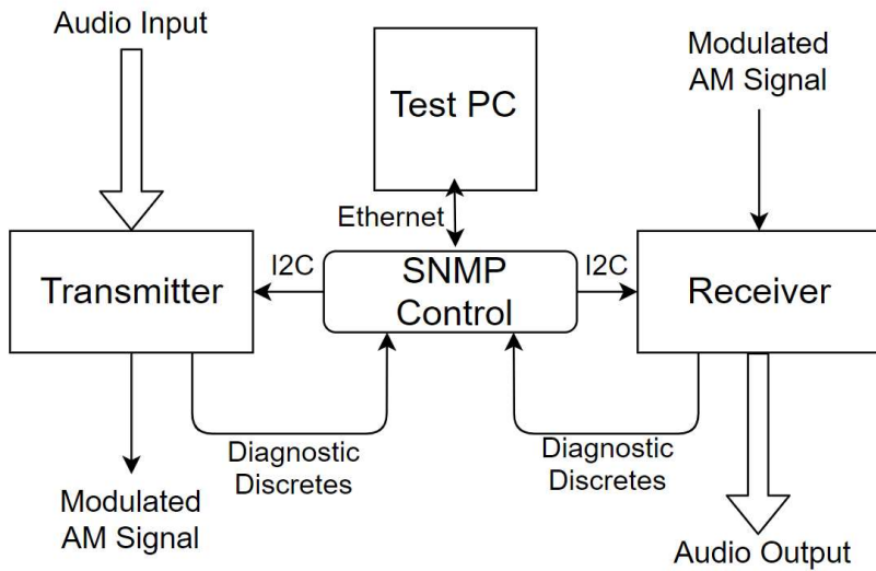
Figure 5: Top-Level Block Diagram
