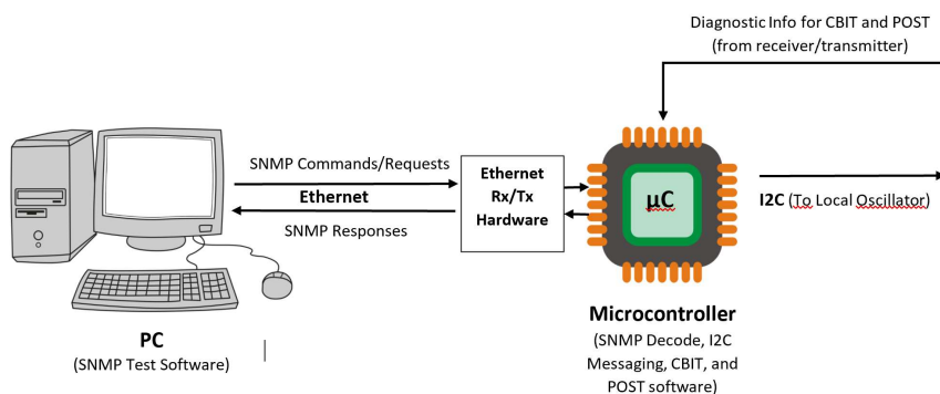
Figure 4: Ethernet Control Circuit
