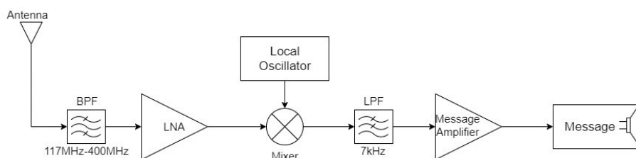
Figure 3: Receiver Block Diagram
